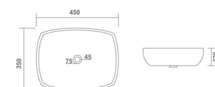
BELLA L 450 W 350 H 120 mm 18" x 14"
