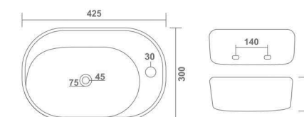
LOGAN L 425 W 300 H 145 mm 17" x 12"
