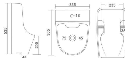
REX L 335 W 305 H 535 mm
