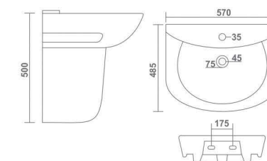
STUDIO L 570 W 485 H 500 mm 23" x 19"
