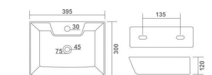
ROB L 395 W 300 H 120 mm 16" x 12"
