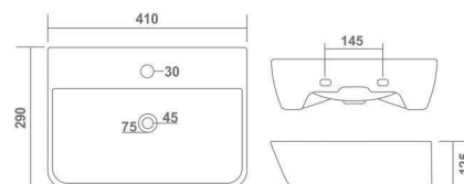
BENZ L 410 W 290 H 125 mm 16" x 12"
