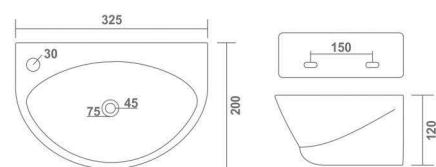
SPOTY L 325 W 200 H 120 mm 13" x 8"
