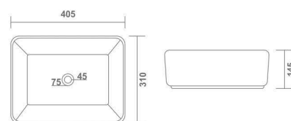
ALEX L 405 W 310 H 145 mm 16" x 12"
