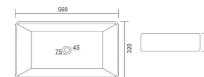
ZORO L 560 W 320 H 140 mm 22" x 13"
