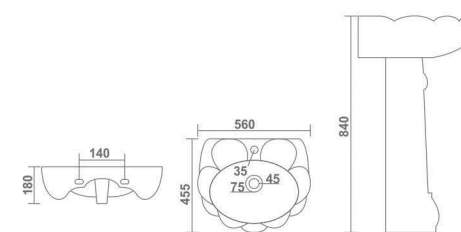
LOTUS L 560 W 455 H 840 mm 22" x 18"
