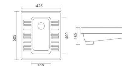
ORISSA PAN FLAT - 21" L 525 W 425 H 225 mm
