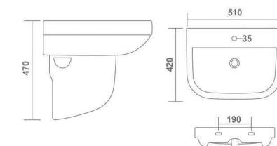
MARVEL L 510 W 420 H 470 mm 20" x 17"
