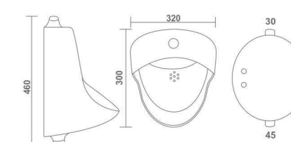
FLAT BACK L 320 W 300 H 460 mm
