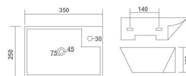
FERRY L 350 W 250 H 120 mm 14" x 10"
