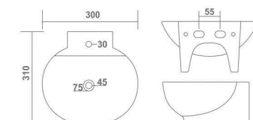
NANO L 310 W 300 H 125 mm 12" x 12"
