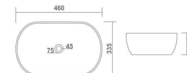
ALIS L 460 W 335 H 145 mm 18" x 13"
