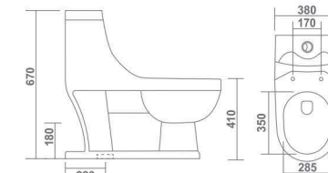
CAMRY L 700 W 380 H 670 mm 'S' Trap : 220mm (9") 'P' Trap
