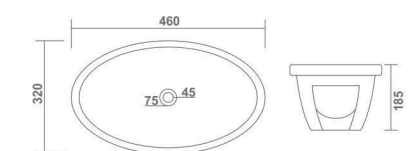
LIZA (Under Counter) L 460 W 320 H 185 mm 18" x 13"
