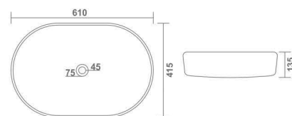
BELLEZA L 610 W 415 H 135 mm 24" x 17"
