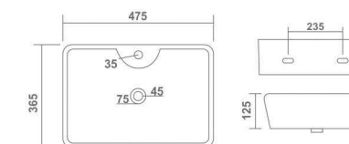
FIONA L 475 W 365 H 125 mm 19" x 15"
