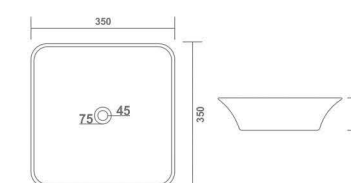
BRUCK L 350 W 350 H 100 mm 14" x 14"
