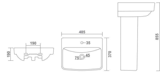
JULIUS L 485 W 370 H 855 mm 19" x 15"
