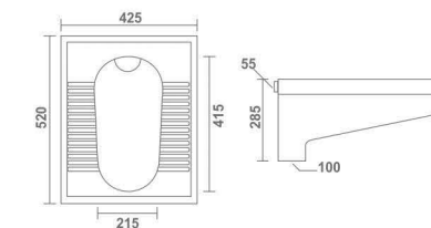
ORISSA PAN - 21" L 520 W 425 H 285 mm
