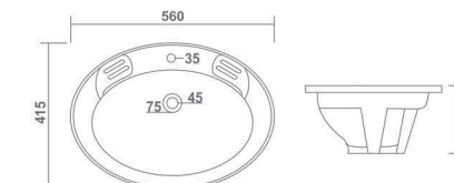
SOBER (Top Counter) L 560 W 415 H 185 mm 22" x 17"
