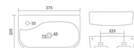
MONTY L 375 W 225 H 120 mm 15" x 9"
