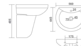
ORCHID L 560 W 445 H 485 mm 22" x 18"
