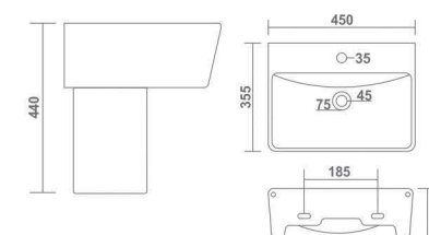
BOOST L 450 W 355 H 440 mm 18" x 14"
