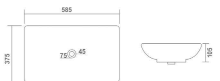
VERO L 585 W 375 H 105 mm 23" x 15"
