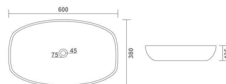
AMAZONE L 600 W 380 H 135 mm 24" x 15"
