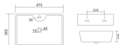
FIONA L 475 W 365 H 125 mm 19" x 15"
