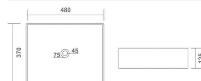
FEMINA L 480 W 370 H 125 mm 19" x 15"
