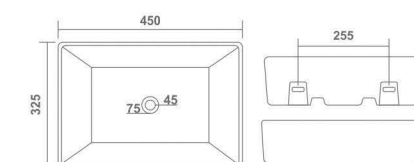
FAST L 450 W 325 H 125 mm 18" x 13"
