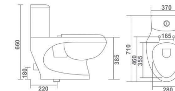
CRISTY L 710 W 370 H 660 mm 'S' Trap : 220 mm (9") 'P' Trap
