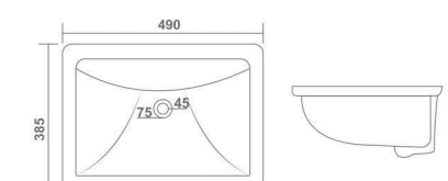
ROMANO (Under Counter) L 490 W 385 H 205 mm 20" x 15"
