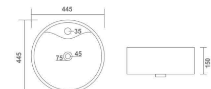
OXO L 445 W 445 H 150 mm 18" x 18"
