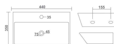
VICTOR L 440 W 350 H 120 mm 18" x 14"
