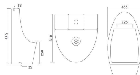
BUZZ L 335 W 310 H 680 mm
