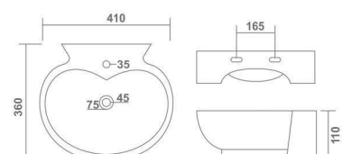
SPIRIT L 410 W 360 H 110 mm 16" x 14"
