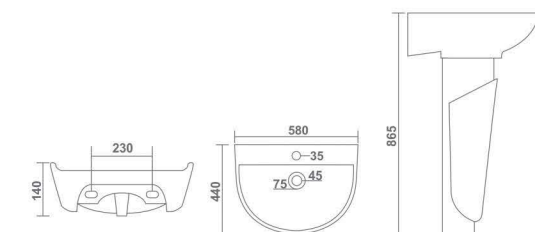
EVA L 580 W 440 H 865 mm 23" x 18"
