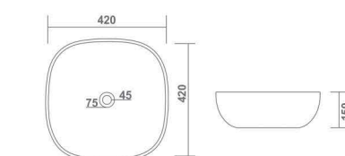
DECOR L 420 W 420 H 150 mm 17" x 17"
