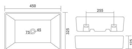
FAST L 450 W 325 H 125 mm 18" x 13"
