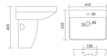
JOLLY L 410 W 335 H 445 mm 16" x 13"
