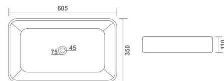
MAGMA L 605 W 350 H 110 mm 24" x 14"
